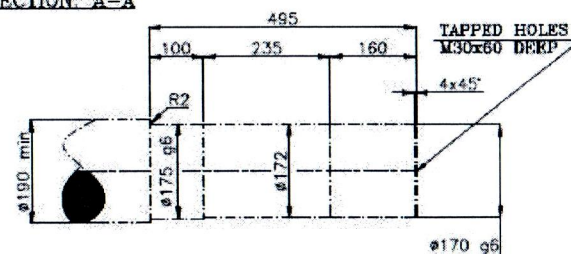
DETAILS OF CUSTOMER O/P SHAFT
